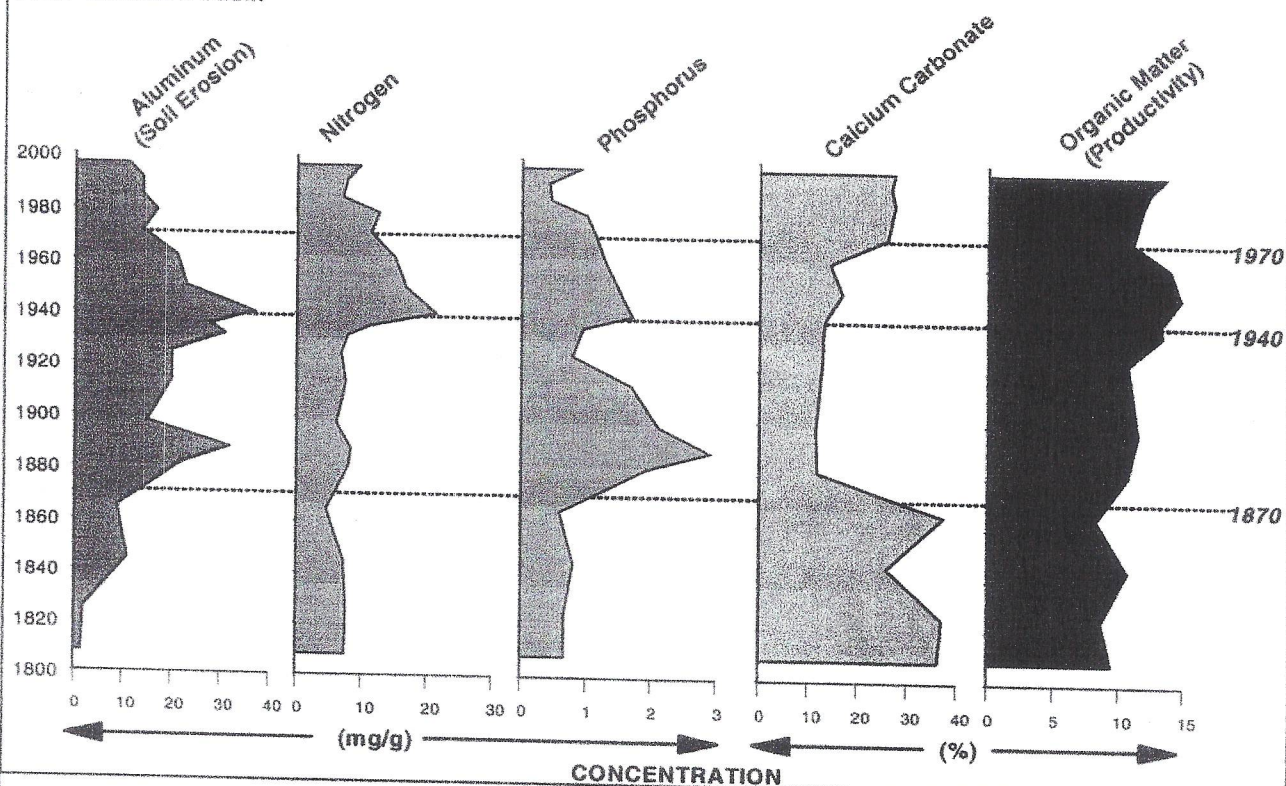
Figure 5. Profiles of selected chemical variables in the core from the south basin. The greatest soil erosion occurred during the period 1880-1950. The rate has been reduced since 1970.
