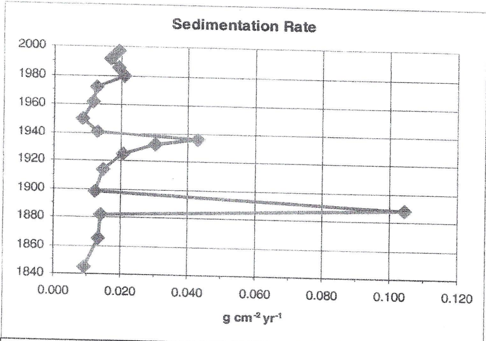
Figure 4. Sedimentation rate for the south basin.
