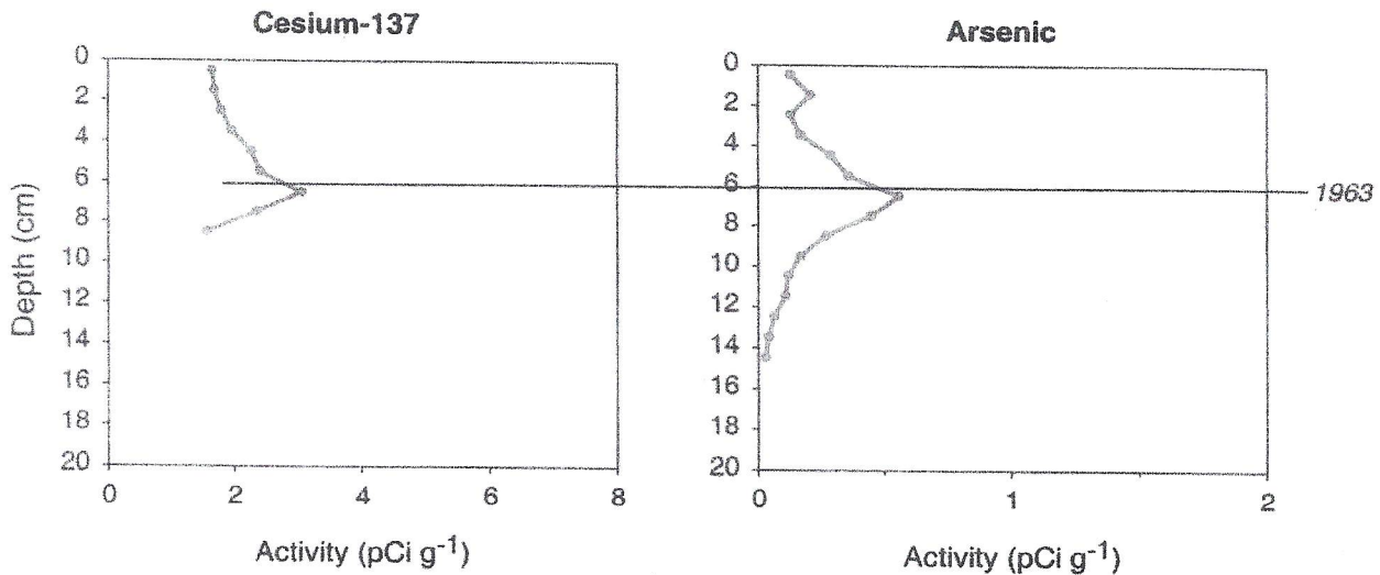
Figure 2. Profiles of cesium-137 and arsenic. Cesium-137 is a byproduct of atmospheric nuclear testing while arsenic was used for aquatic plant control in the 1950-60s. The peak deposition of both of these chemicals in Big Cedar Lake was 1963.
